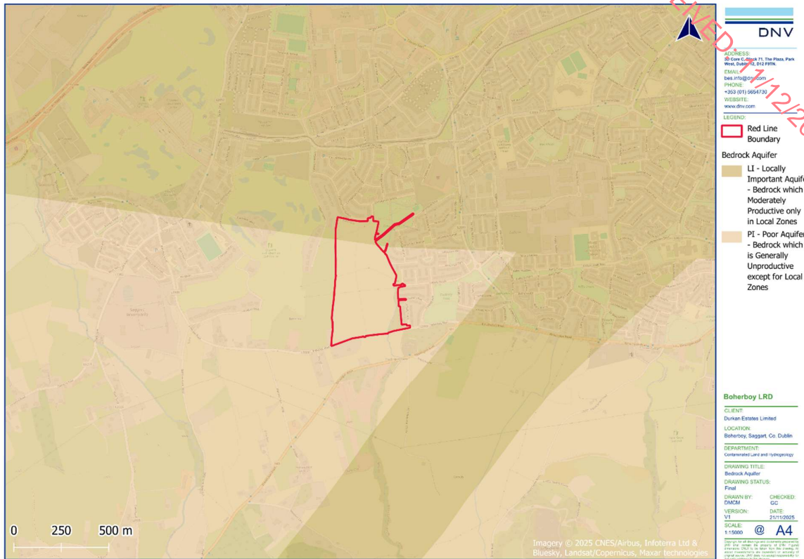
Figure 4-4. Bedrock Aquifer
