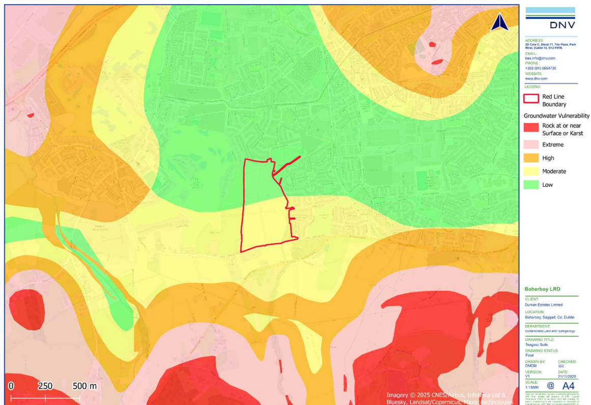
Figure 4-5. Groundwater Vulnerability
