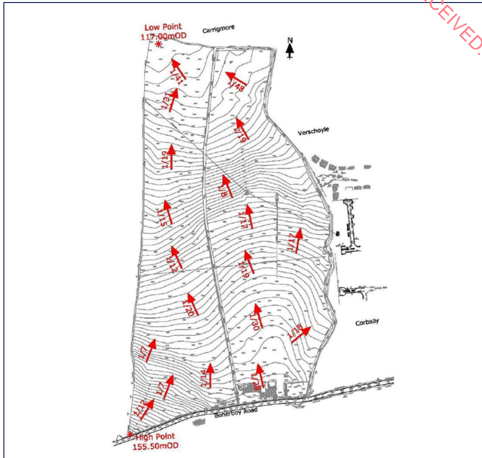
Figure 3-3. Existing Topography (Extract from Roger Mullarkey & Associates, 2025. Drainage and Water Infrastructure Engineering Report)
