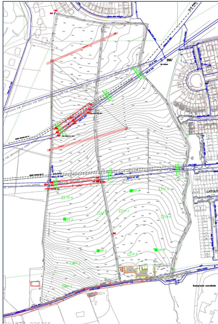
Figure 4-6. Site Investigation Locations (Extract from GII, 2014)
