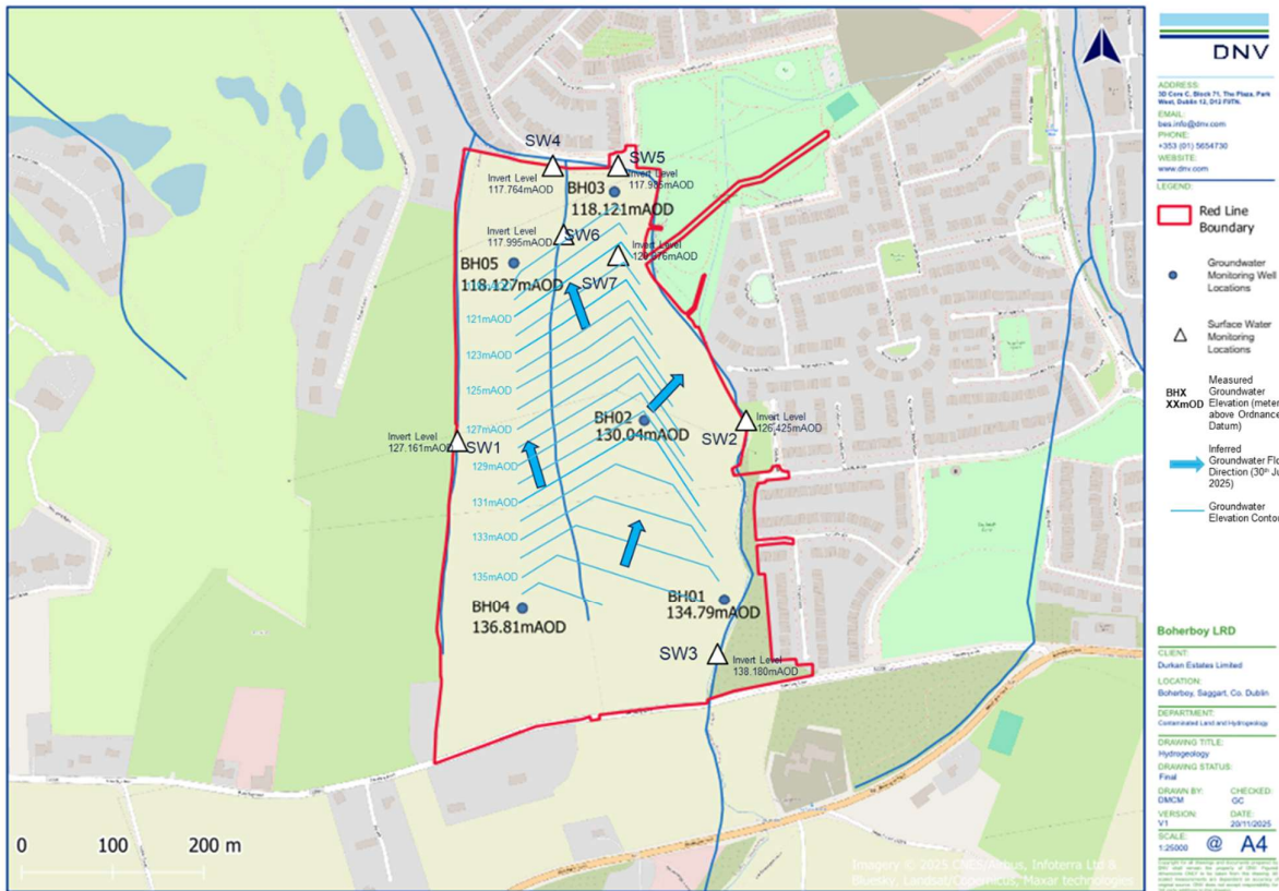
Figure 6-1. Inferred Groundwater Flow Direction (30/06/2025)
