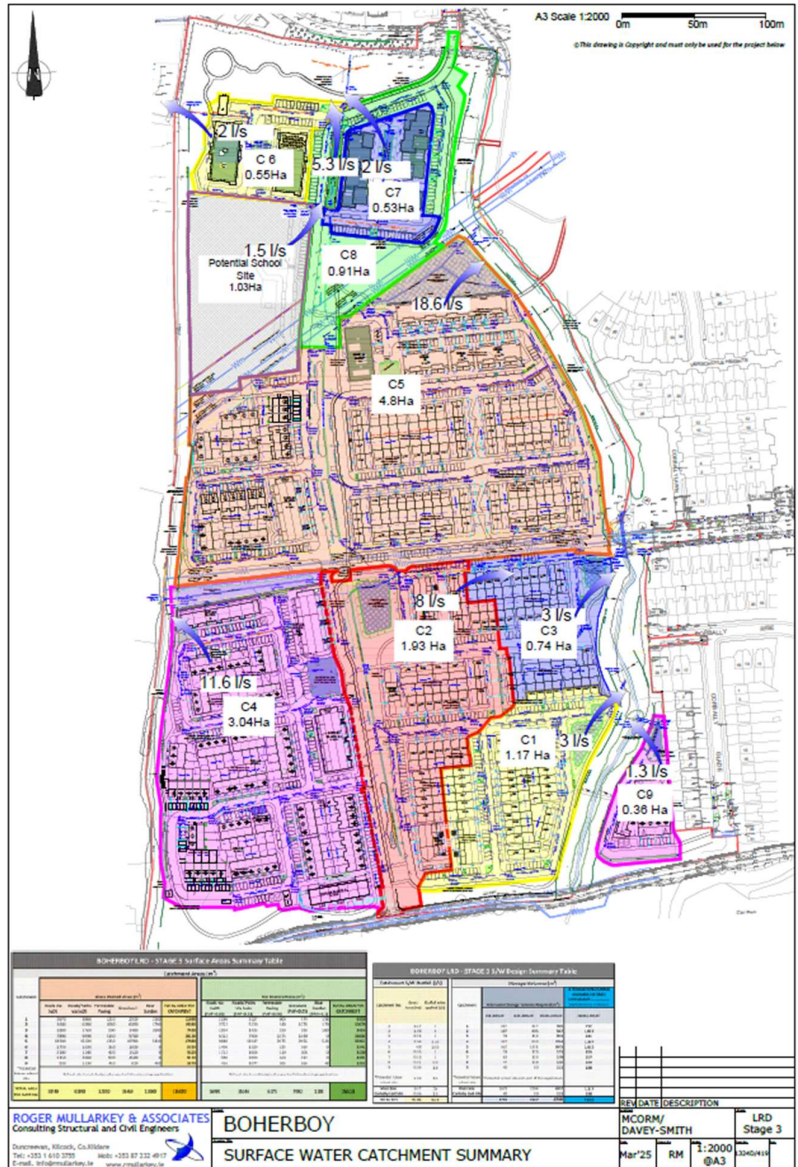
Figure 3-4. Surface Water and Groundwater Catchment Summary (Roger Mullarkey & Associates, 2025)
