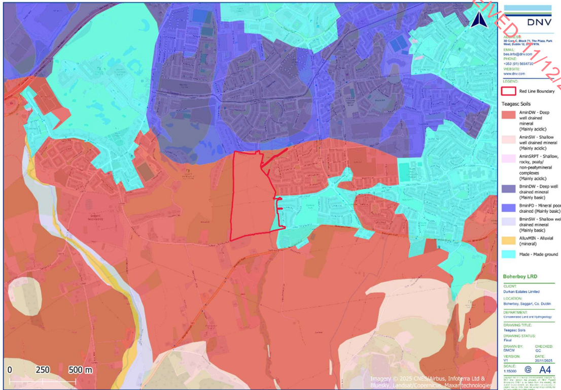
Figure 4-1. Teagasc Soils
