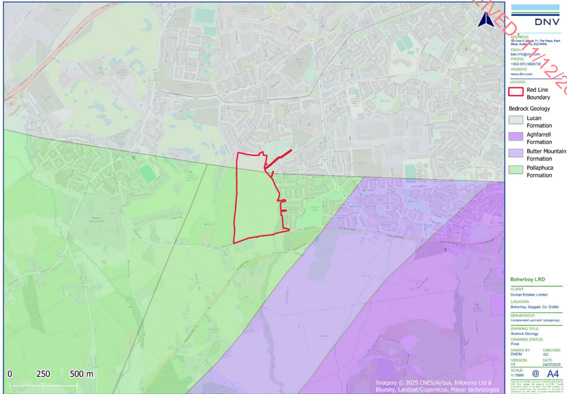
Figure 4-3. Bedrock Geology
